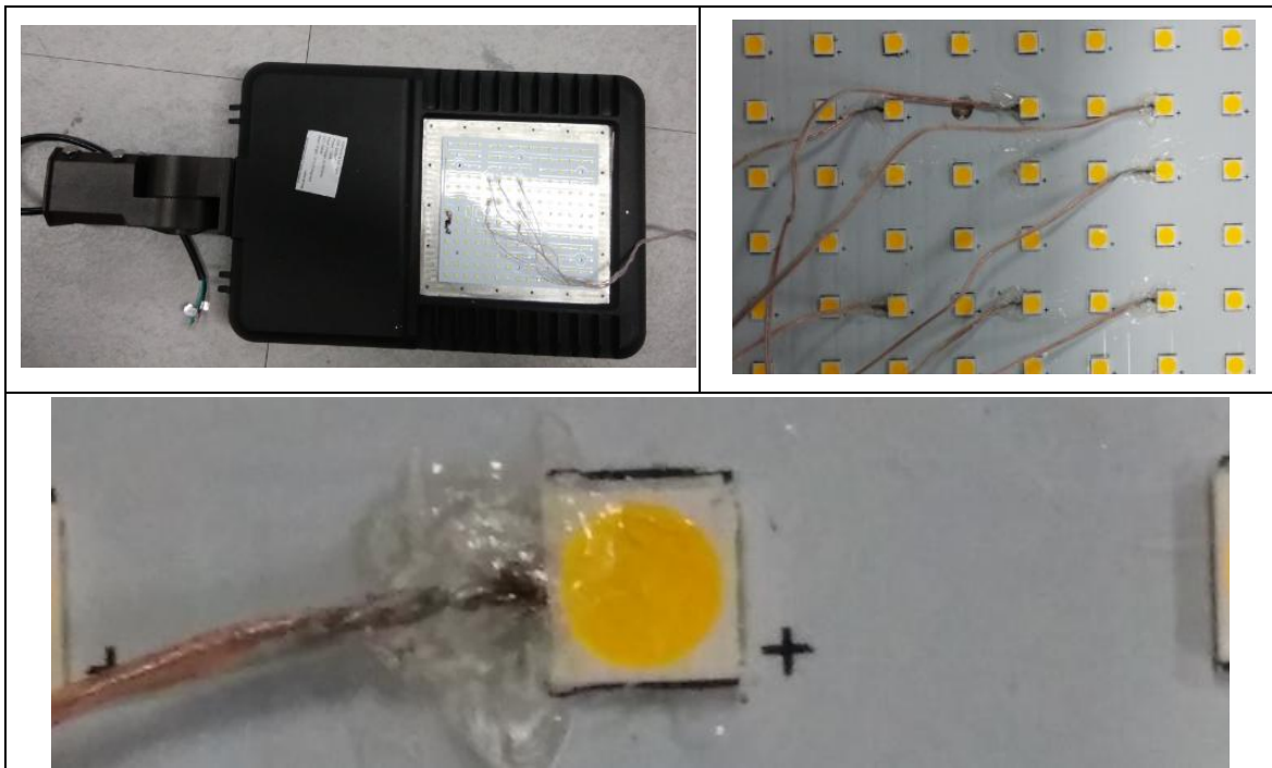
Thermocouple Location on Temperature Measurement Point (TMP):
