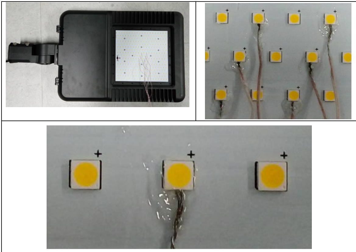
Thermocouple Location on Temperature Measurement Point (TMP):
